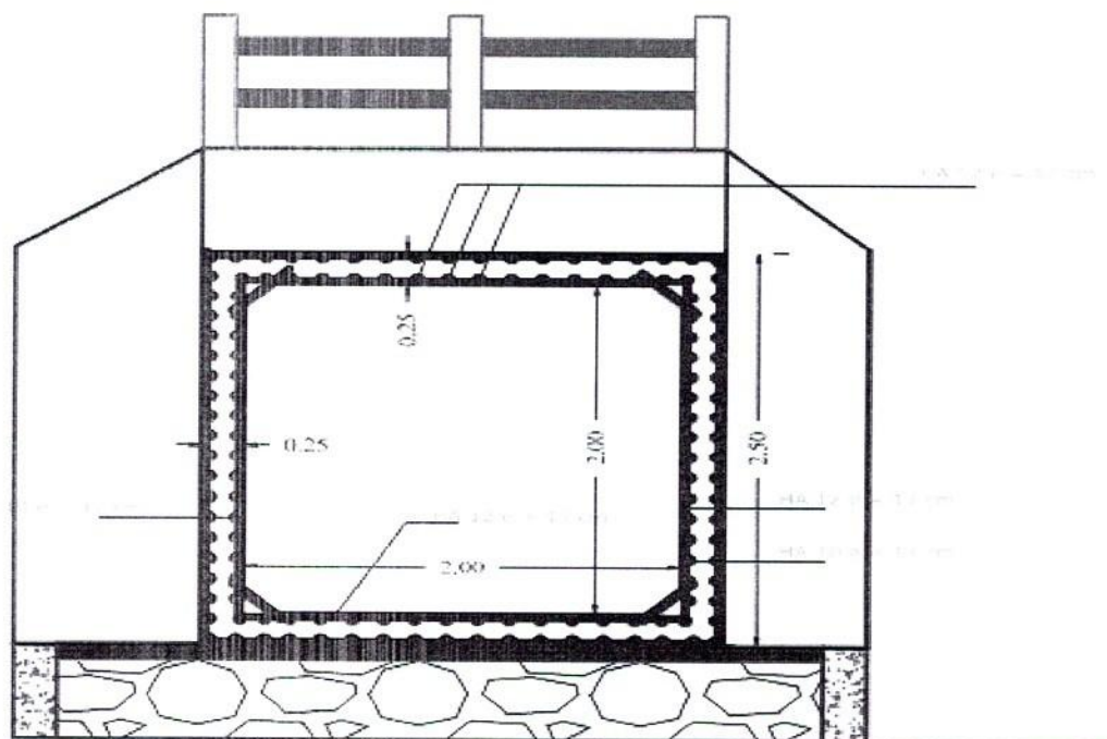
REINFORCEMENT SECTION A-A
